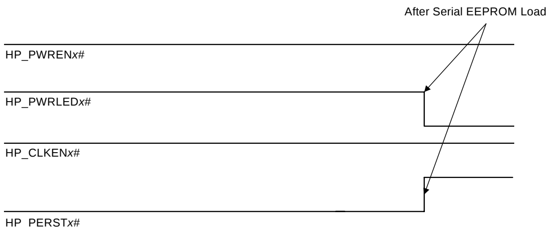
Figure 11-2. Hot Plug Outputs when Power Controller Present and Power Controller Control Bits Are Cleared
